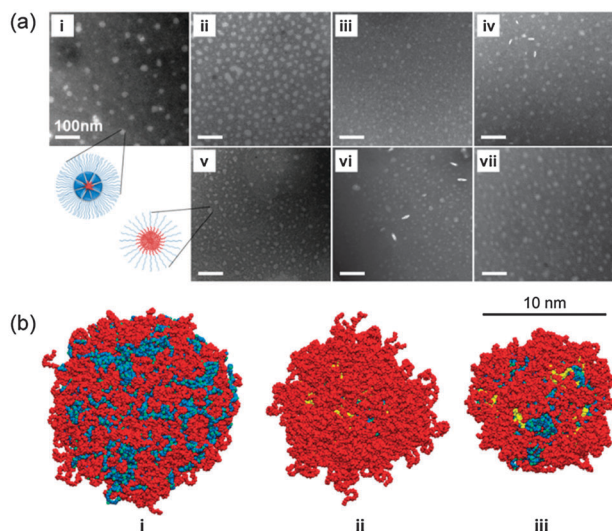
Fig. 3 (a) TEM images of micelles self-assembled from PDCs: (i) PCL3.5K-G3-mPEG2K, (ii) PCL3.5K-G3-mPEG5K, (iii) PCL14K-G3-mPEG2K, (iv) PCL14K-G3-mPEG5K; and from the linear copolymers: (v) PCL3.5K-mPEG2K, (vi) PCL3.5K-mPEG5K, and (vii) PCL14K-mPEG5K. Scale bar = 100 nm. (b) MD simulations of micellar structures formed from (i) 128 PCL3.5K-mPEG2K, (ii) 14 PCL3.5K-G3-mPEG2K, and (iii) 10 PCL14K-G3-mPEG2K (PCL: blue, G3-dendron: yellow, PEG: red). Water is not shown.
