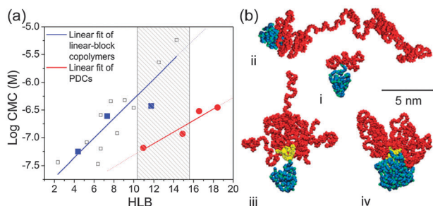
Fig. 2 (a) Linear relationship between CMC and HLB for (●) PDCs and (■) linear-block copolymers. Additional data points for the linear-block copolymers (□) were acquired from the literature that used the same polymer blocks. Note that, at the same HLB (10–15), the PDC self-assemblies maintain CMCs that are 1–2 orders of magnitude lower than the linear counterparts, as highlighted in the shaded region. (b) MD simulations of (i) PCL3.5K-mPEG2K, (ii) PCL3.5K-mPEG16K, (iii) PCL3.5K-G3-mPEG2K, and (iv) PCL14K-G3-mPEG2K molecules after 5 ns in water (PCL: blue, G3-dendron: yellow, PEG: red). Water is not shown.
